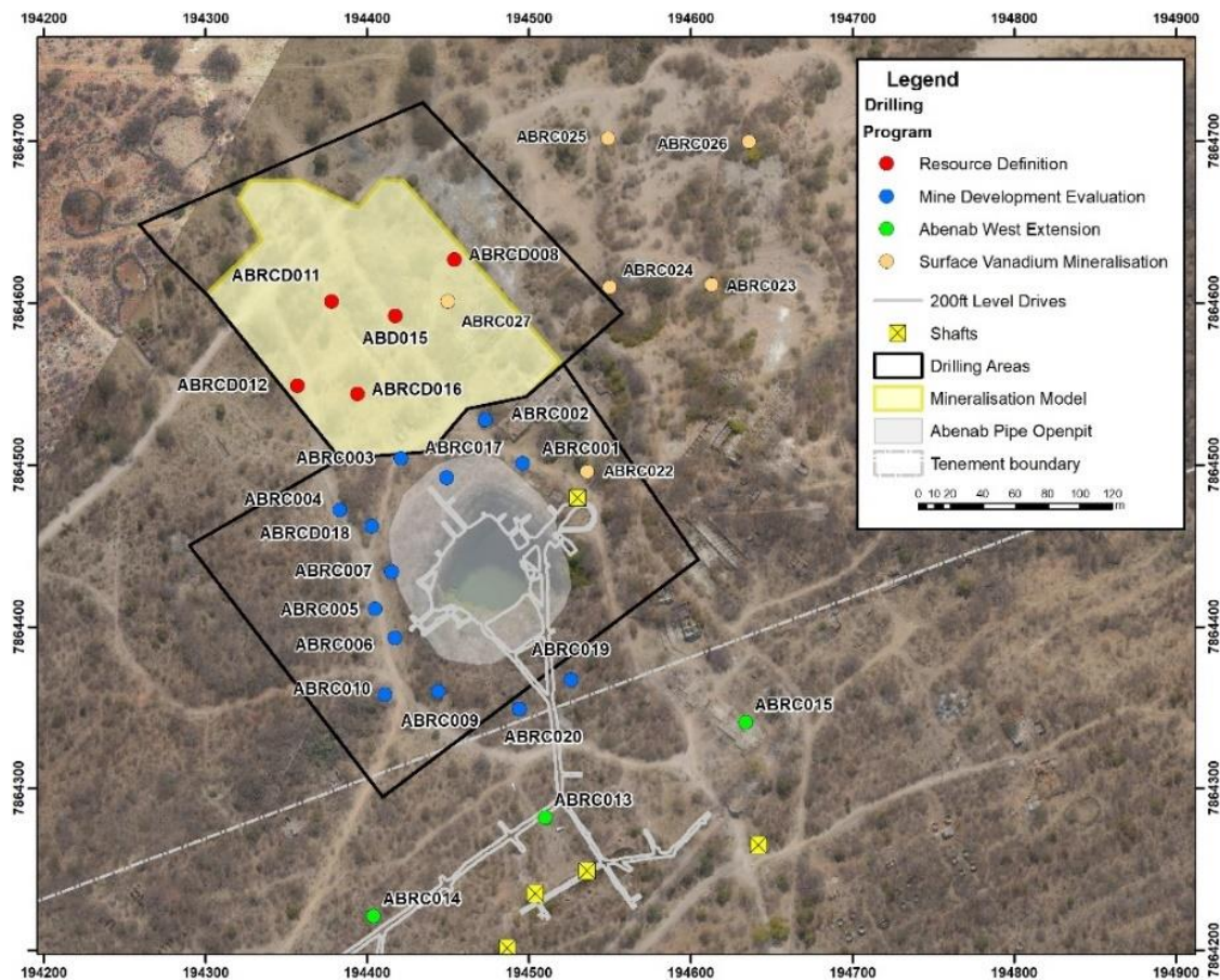
Figure 1: Phase 1 drilling completed at Abenab Mine
