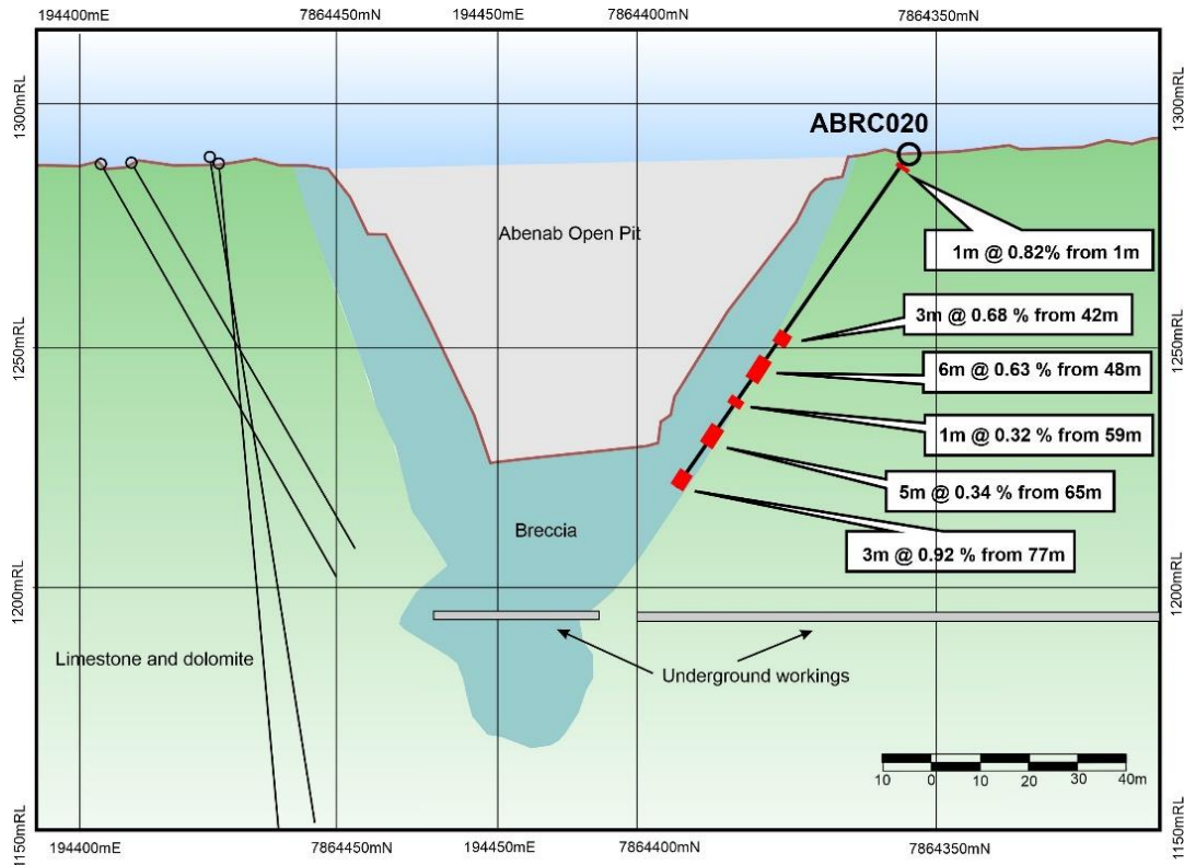
Figure 2: Cross section showing vanadium mineralisation in RC hole ABRC020
