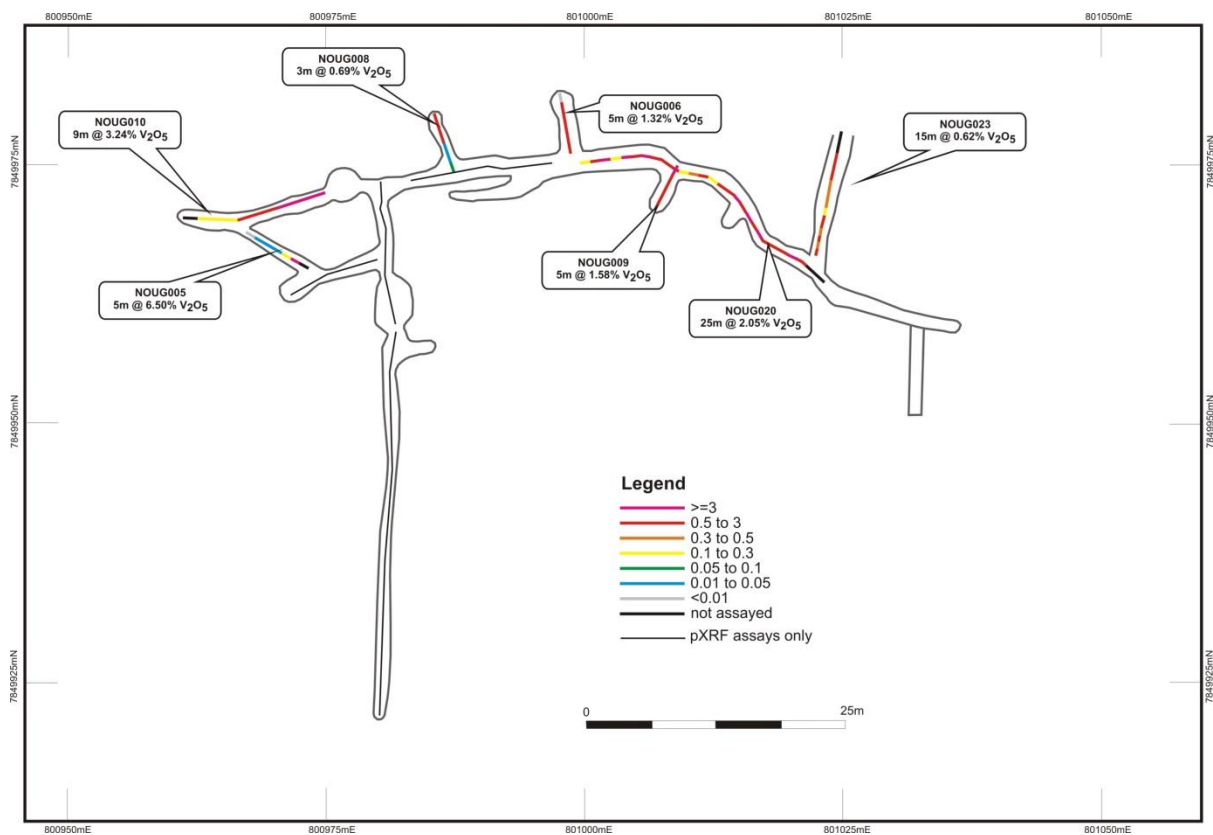
Figure 10: Nosib Block prospect Level 1. Vanadium pentoxide channel sample results.
