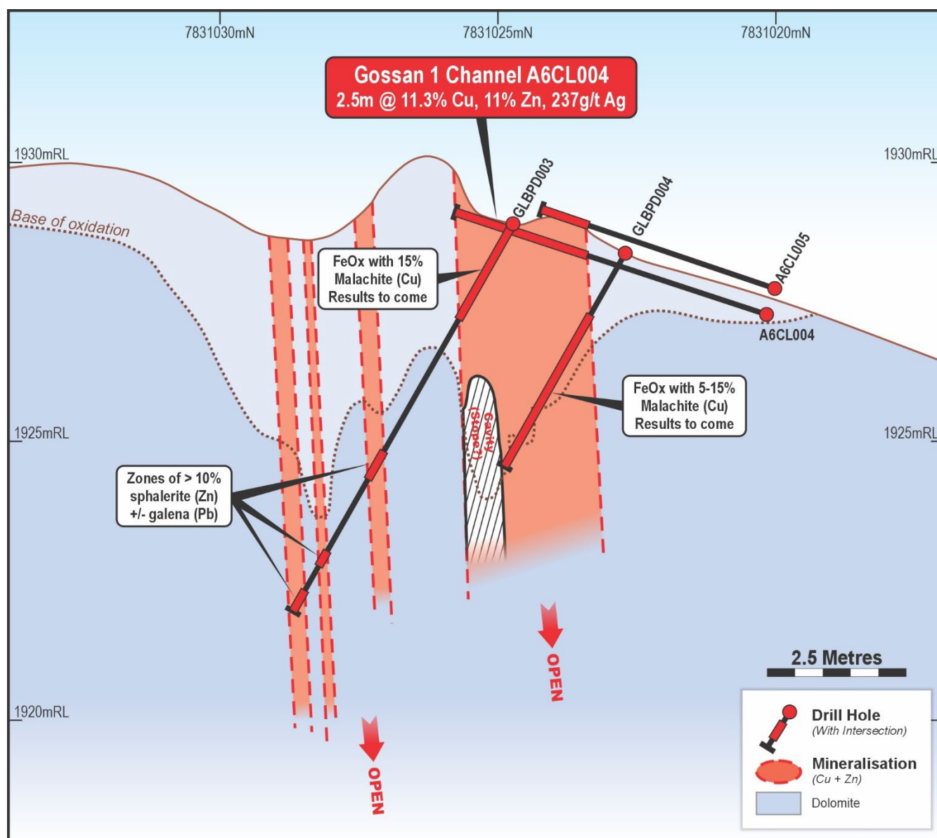
Figure 3: Cross section through Gossan 1, 796,416.5mE, showing previous channel intersections and drillholes GLBP003 & 004
