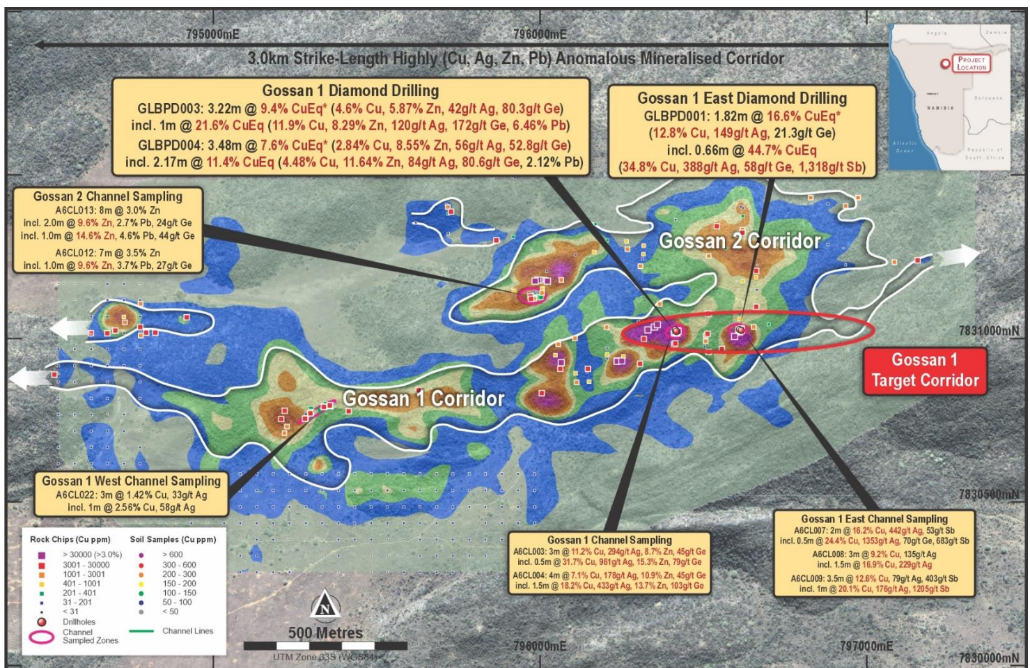
Figure 7: Graceland mineralised corridor, with channel & drilling intersections, on copper soil contours and rockchip samples
