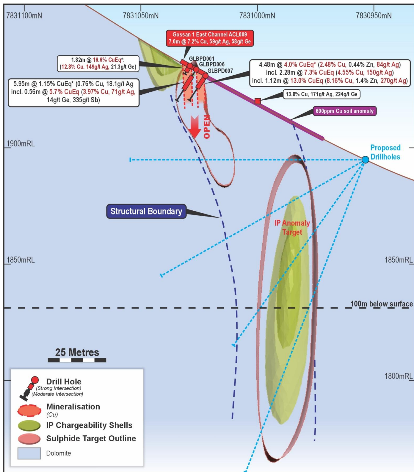
Figure 4: Graceland, cross section 796,620mE, showing Gossan 1 East shallow drilling intersections & planned drilling to test the IP Sulphide Target
