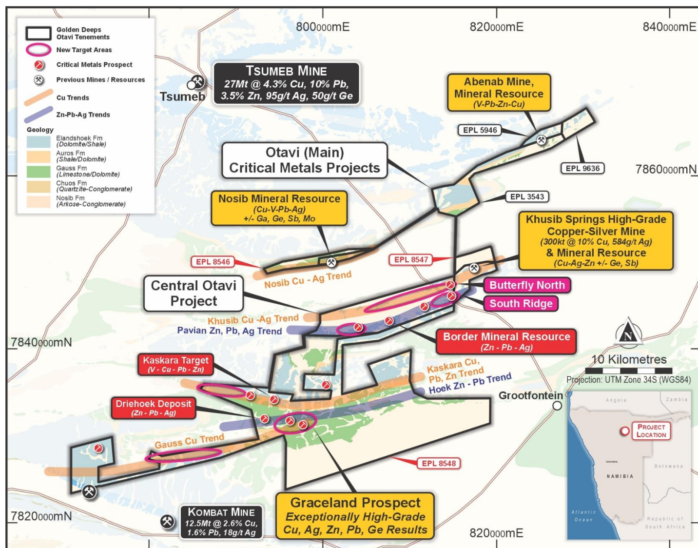
Figure 6: Golden Deep's Otavi Critical Metals Project showing key prospects, "Tsumeb-type" target areas and the Graceland Prospect
