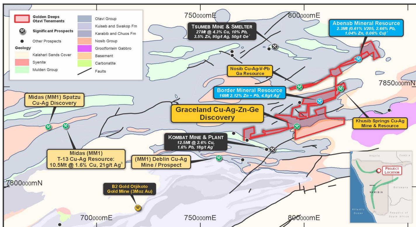
Figure 5: Golden Deeps Otavi Mountain Land Projects and key prospects as well as major mines and resources in the region
