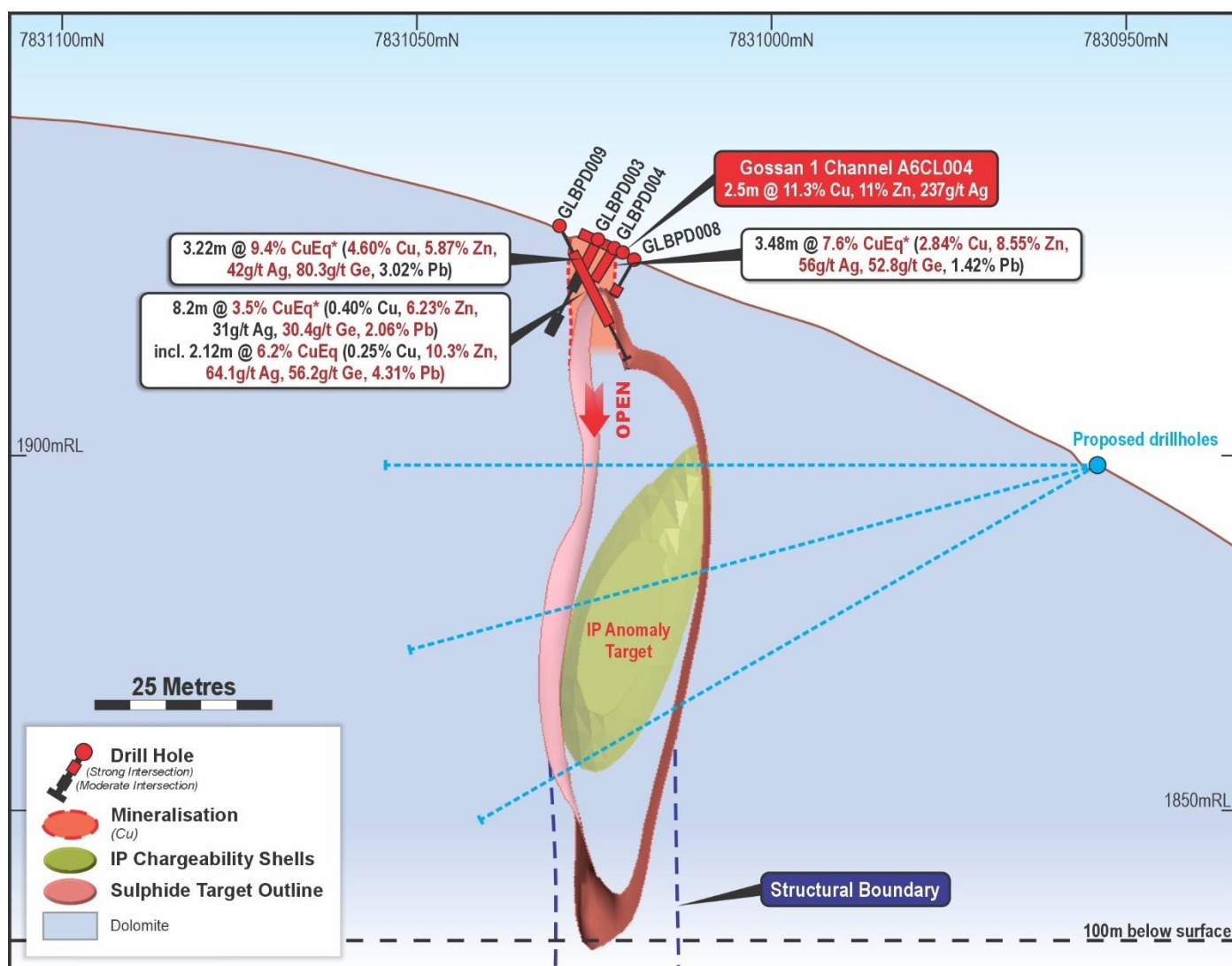
Figure 3: Graceland, cross section 796,420mE, showing Gossan 1 shallow intersections & planned drilling to test the IP Sulphide Target
